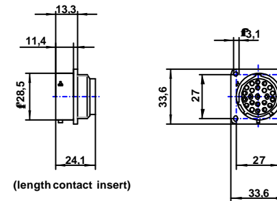
Receptacle with female contacts enclosed
